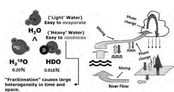
水の安定同位体と地球水循環とのかわり Schematic illustration of stable water isotopes and their relation to the Earth's water cycle
